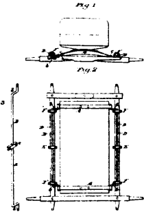
13269 Magnier & Thomas's Improvements on Vehicle Springs.
