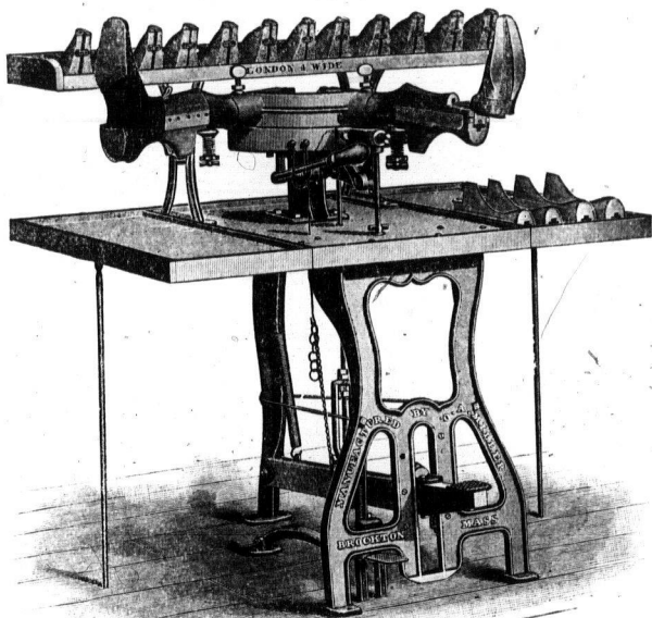
The Miller "Twin" Shoe Treeing Machine.
