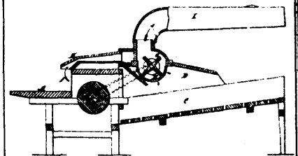
2274 Hunsberger &amp; Latshaw's Dust Conveyor for Threshing Machines.
