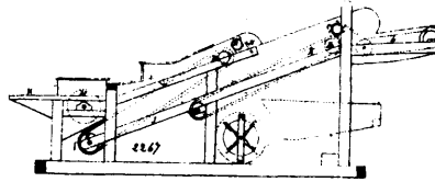
2267 Brothers &amp; Downs' Threshing Machine.
