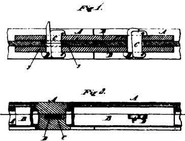
2268 Braymer's Railroad Fish Plate Fastener.
