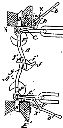
24218 Copland & Gilmour's Car Coupling.
