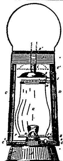
24219 Kennedy's Tubular Lantern
