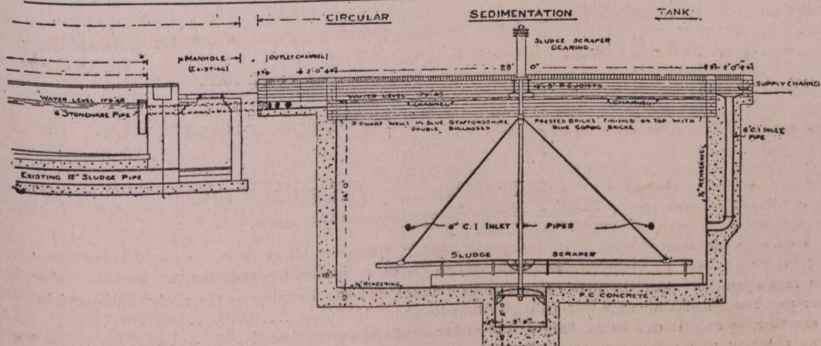
Section of Circular Sedimentation Tank.
