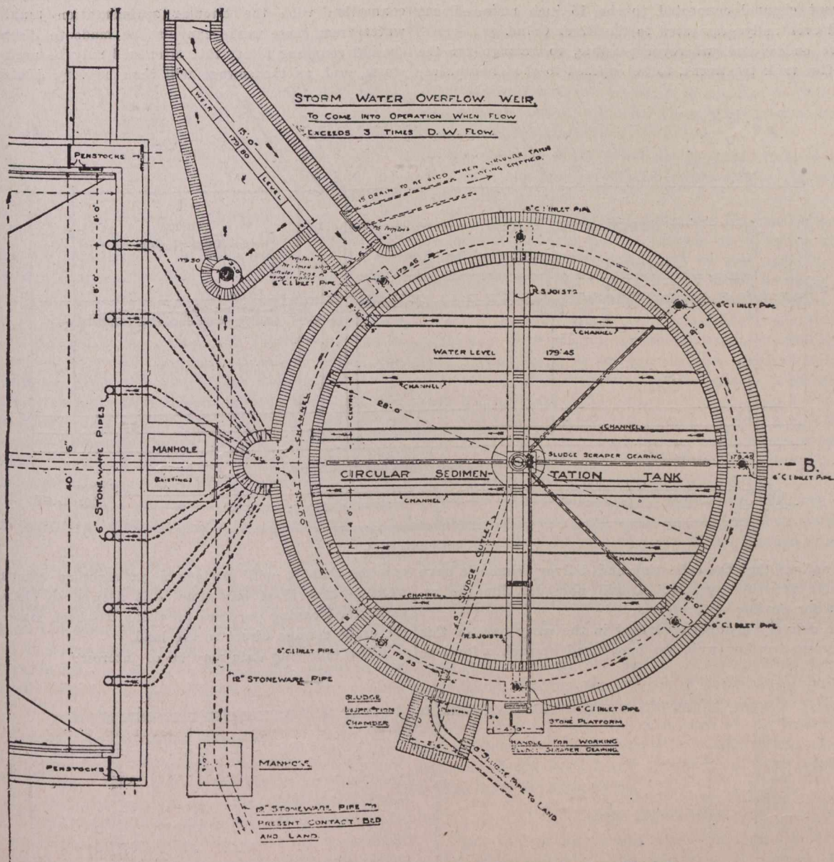
Plan of Circular Sedimentation Tank, Bushey Sewage Works.
