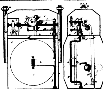
2844 Telling & Johnson's Dry Gas Meter.
