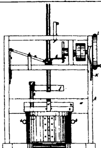
2850 Stockwell's Machine for the Manufacture of Cement Pipes.
