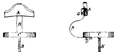
2854 Bolton's Improved Double Adjustable Piano Stool Back.
