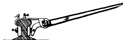
2848 Baker's Bolt Holder for Railroad Rails.
