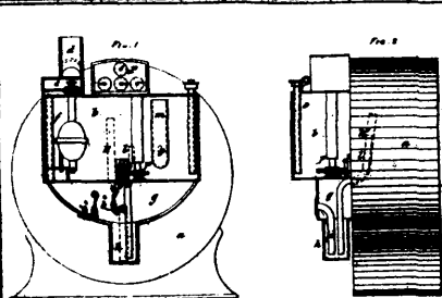
2843 De Castro & Burton's Compensating Wet Gas Meter.
