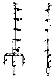
6982 Shelton's Improvements in Fence Posts.
