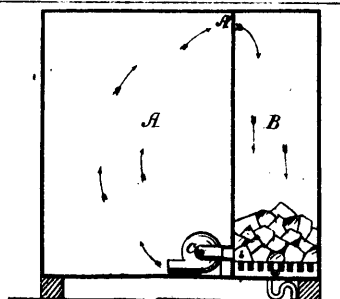
6991 Bate's Improvements on Refrigerators.
