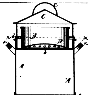
6985 Brooks' Improvements in Coal Ash Sifters.
