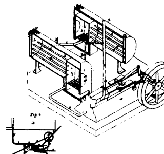
4449 Mosman's Method of Generating and Utilizing Steam.
