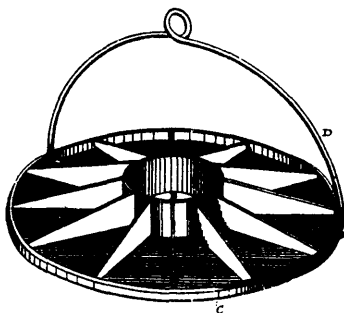
4445 Thompson's Face-tester for Mill-stones.
