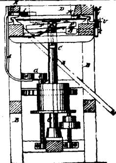
1987 Anderson, Gue &amp; Utley's Shingle Machine.
