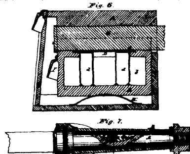
1988 Eggleston's Device for Lubricating Car and Carriage-Axes.
