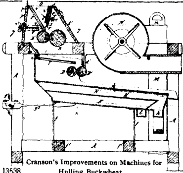
13538 Cranson's Improvements on Machines for Hulling Buckwheat.
