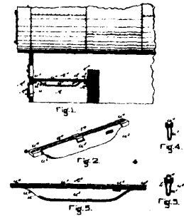
13537 Fairbairn's Improvements on Grate Bars.
