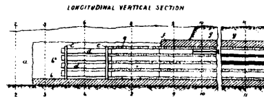
13542 Derrick's Improvements in Continuous Underground Pipes.
