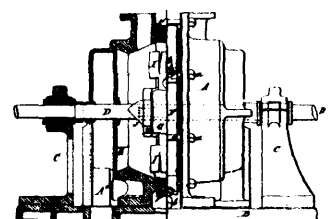
13549 Cook's Pulverizing Machine.
