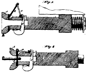
13534 Grant's Improvements on Car-couplings.
