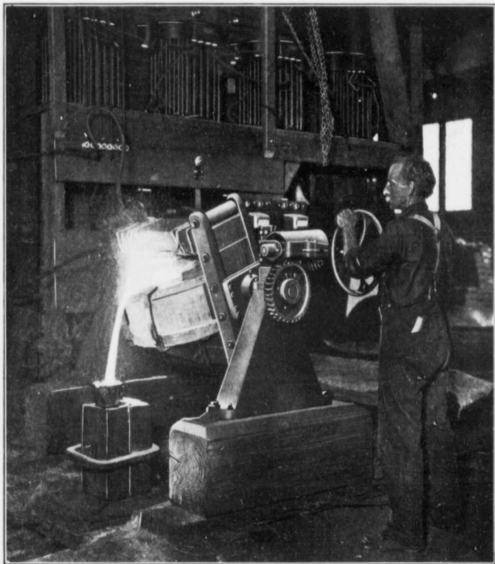
COLBY ELECTRIC STEEL FURNACE
