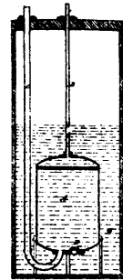
13340 Brewer's Improvement on Water Lifters.
