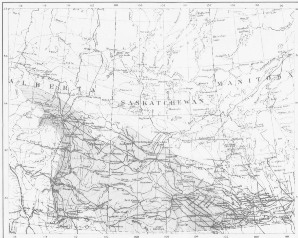
Structure contours showing Gas Horizon near base of Colorado Group.
