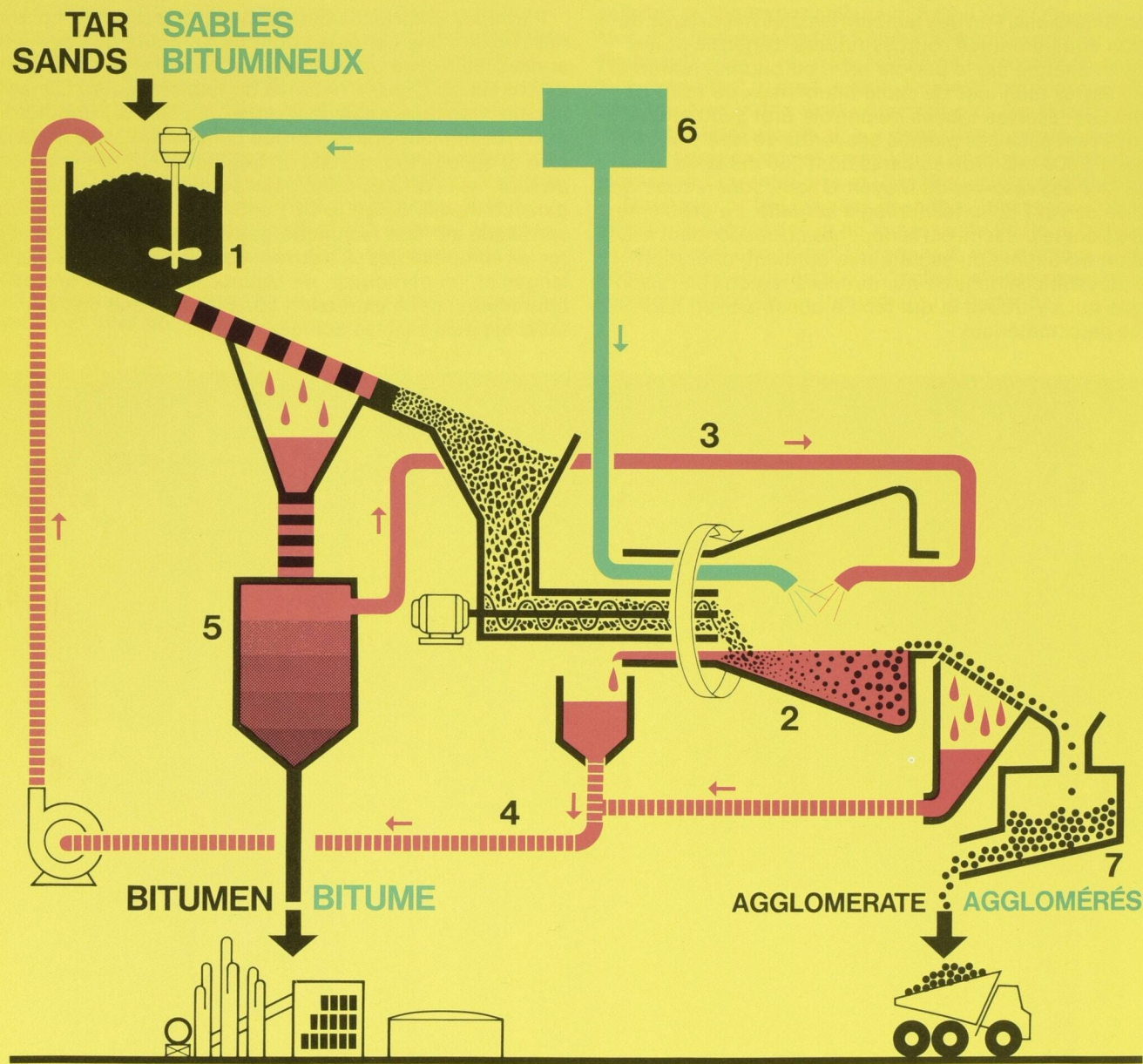
SCHEMATIC DIAGRAM SHOWING EXTRACTIVE AGGLOMERATION OF TAR SANDS
