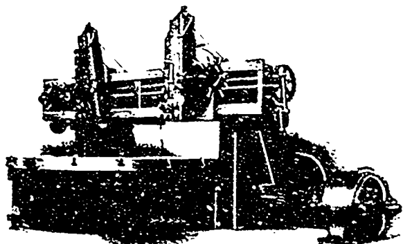
60 in. Horizontal Boring Mill.
