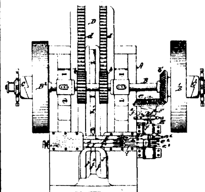
Bird's Pitchfork Making Machine.
