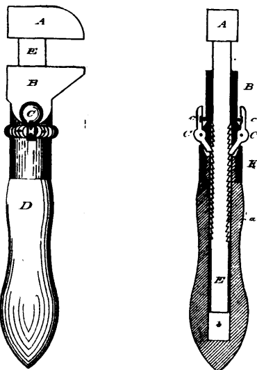
Hadley and Merrill's Wrenches.
