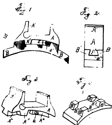
Curtice's Brake Shoes.
