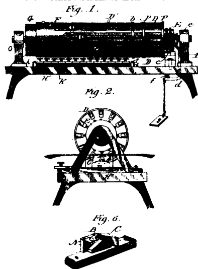
Dement's Type Writing and Printing Machine.
