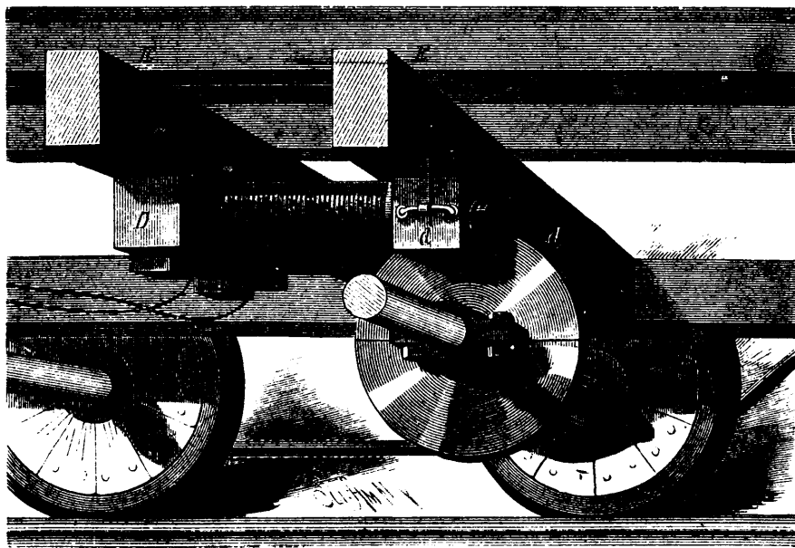
EDISON'S ELECTRO-MAGNETIC BRAKE.
