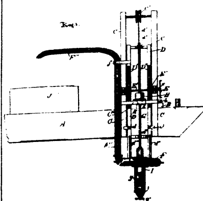
34353 Allison &amp; Nash's Device for Raising Sand from Water.
