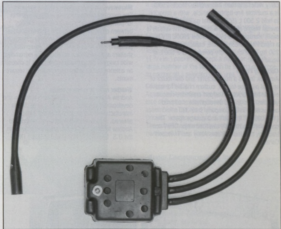
Polychloroprene encapsulated isolating transformer with earthing stud
