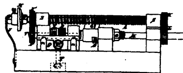
4105 Ross' Machine for Finishing Horse Shoe Nails.
