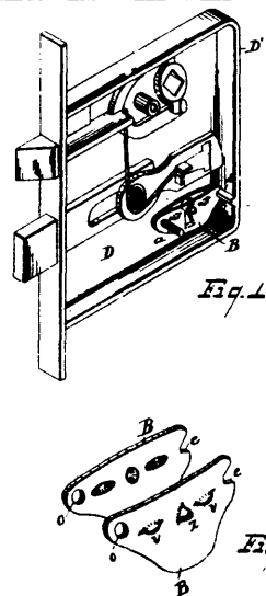
32568 Stoddard's Lock Case Attachment.
