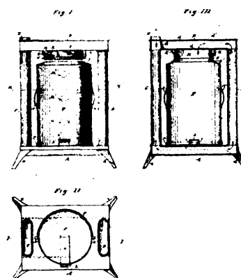
32562 Laube's Straw-Burning Stove.
