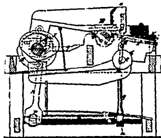
3323 Dodge's Cold Finishing Nail Machine.
