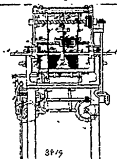
3819 Cooper, Clarke, Donisthorpe & Corap's Knitting Machine.
