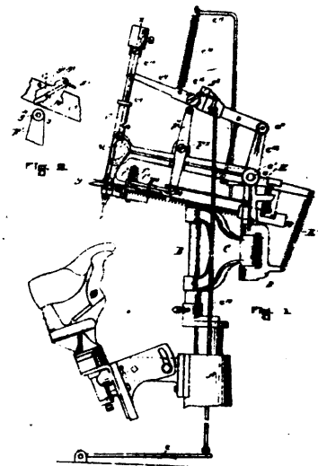
21547. Woodward's Tacking Machine for Lasting Boots and Shoes.
