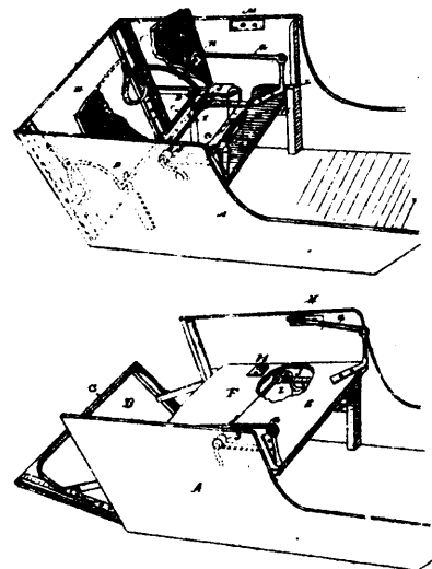
21544. Penfold's Adjustable Seat for Vehicles.
