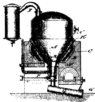
40733 Domeier and Hagemann's Apparatus for Distilling Glycerine Recovered from Soap Lye.
