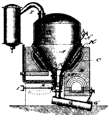
40732 Domeier and Hagemann's Apparatus for Distilling Glycerine Recovered from Soap Lye.
