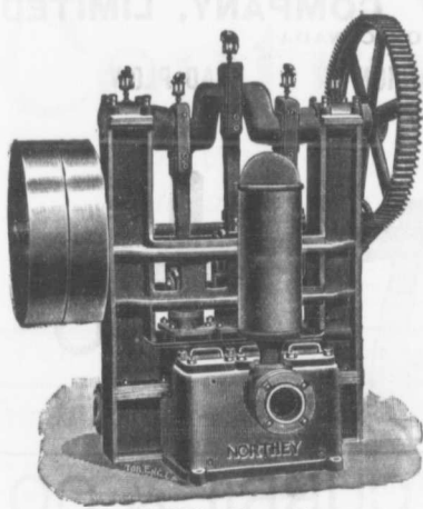
Class B Triplex Power Pump.
