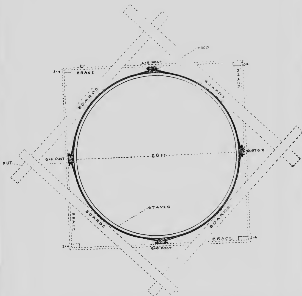
FIG. 3. — Plan of scaffolding that may be used when posts are employed instead of clips to hold the hoops in position. The 2 x 4 pieces are temporary posts supporting braces at intervals. Boards resting upon the braces form scaffolding.
