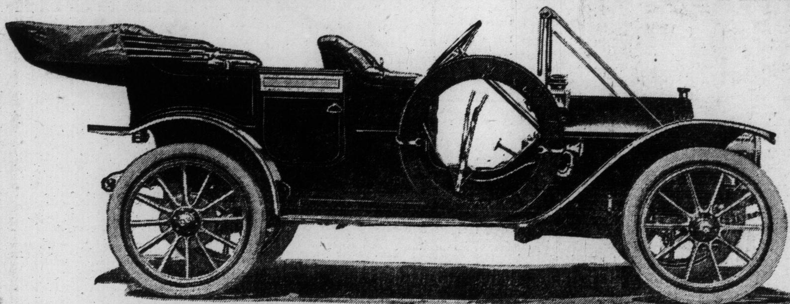
"EVERITT" STANDARD TOURING 1911 MODEL, $1,450. Double-drop frame, 110 in. wheel base, 56-in. gauge, 34 in. wheels, 3½ in. tires, universal rims, internal and external brakes on rear wheels, Bosch high-tension magneto, improved adjustable cone clutch, selective speeds, 3 forward, 1 reverse. Motor: 4 cylinder, 4 cycle, long stroke en bloc, 4 in. x 4½, self-lubricating. Equipment: magneto, horn, 5 gas and oil lamps, generator, extra tire, tire cover, brackets, foot-rest, robe-rail, shock absorbers and tool kit. (Molair top, dust cover and windshield, $125.00 extra.) F.O.B., Orillia.
