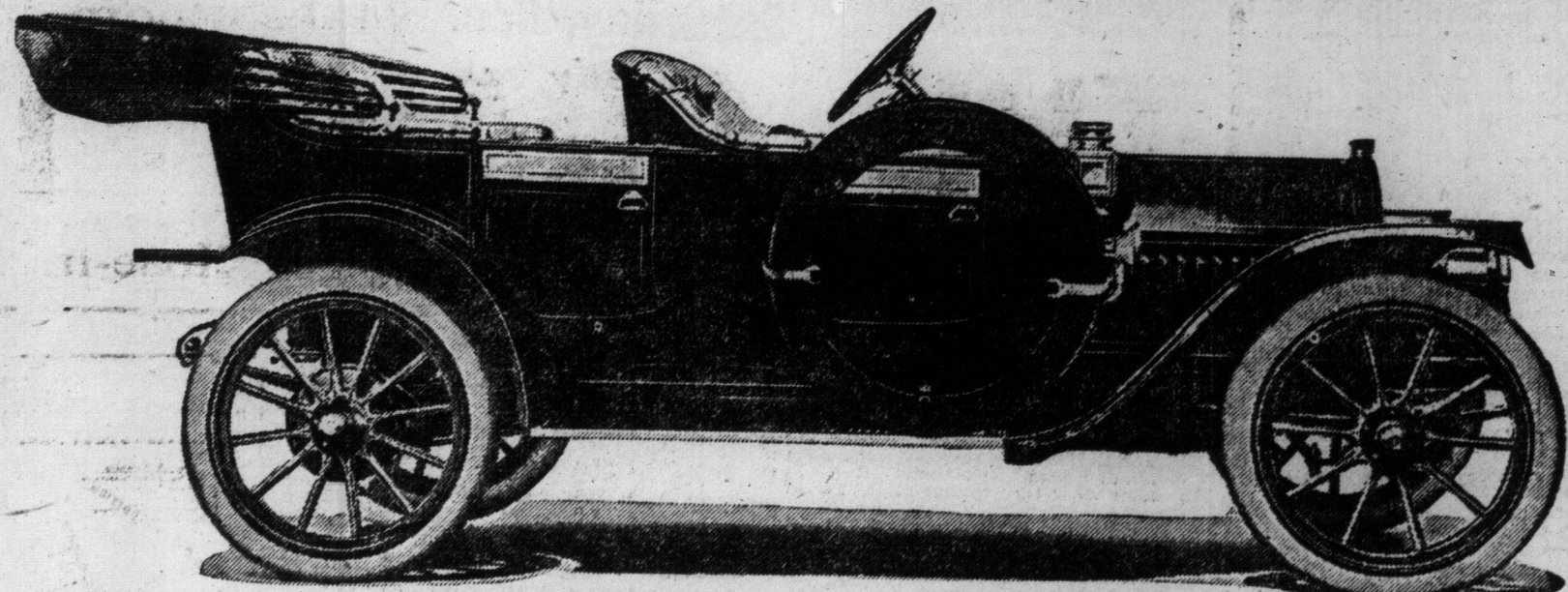
"EVERITT" FORE DOOR TOURING 1911 MODEL, $1,500. Double-drop frame, 110 in. wheel base, 56-in. gauge, 34 in. wheels, 3½ in. tires, universal rims, internal and external brakes on rear wheels, Bosch high-tension magneto, improved adjustable cone clutch, selective speeds, 3 forward, 1 reverse. Motor: 4 cylinder, 4 cycle, long stroke en bloc, 4 in. x 4½, self-lubricating. Equipment: magneto, horn, 5 gas and oil lamps, generator, extra tire, tire cover, brackets, foot-rest, robe-rail, shock absorbers and tool kit. (Molair top, dust cover and windshield, $125.00 extra.) F.O.B., Orillia.
