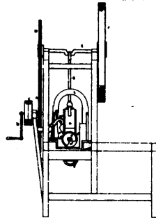
3768 Wallace's Improvements on Machines for Making Matches.
