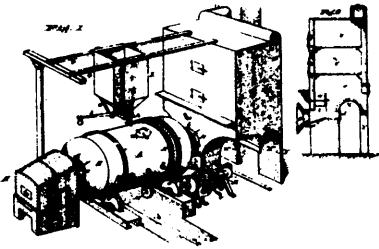
3764 Teats' Ore Roasting Furnace.
