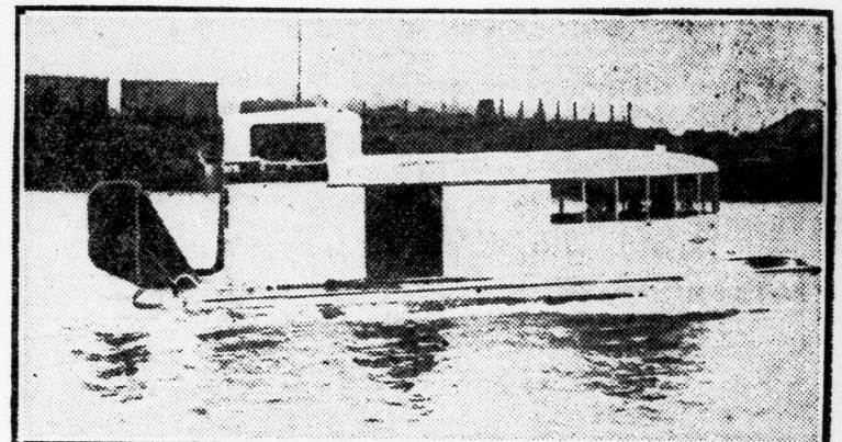
Hydro-glider, made in Belgium for work in the shallow waters of the Congo river, Africa. It carries merchandise and six passengers at 40 kilometres an hour.
