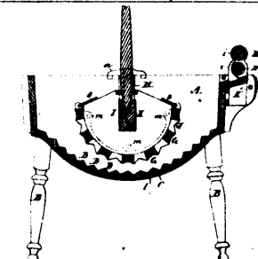
13019 Cahoon's Improvements on Washing and Wringing Machines.
