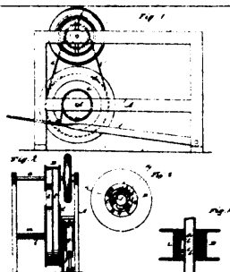
13024 Mayo &amp; Perry's Improvements on Foot Power Mechanism.
