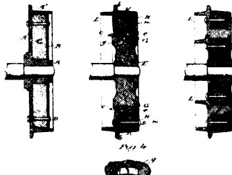
13018 Taylor's Improvements on Car Wheels.
