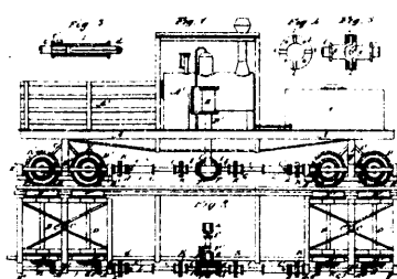
13017 Shay's Improvements in Locomotive Engines.
