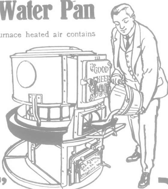
SKELETON VIEW OF "GOOD CHEER" FURNACE SHOWING BIG "CIRCLE WATER PAN"
