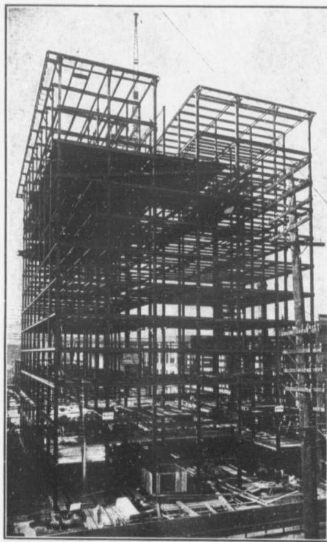
STEEL FRAME, ROYAL CONNAUGHT HOTEL BUILDING, FABRICATED AND ERECTED BY THE HAMILTON BRIDGE WORKS CO., LTD. WEIGHT OF STEEL, 1,440 TONS.
