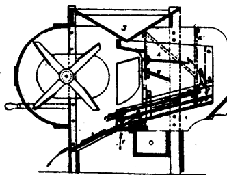
7289 Bennett's Improvements on a Fanning Mill.
