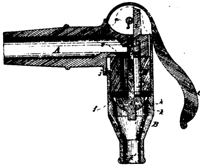
2339 Smith's Faucet.
