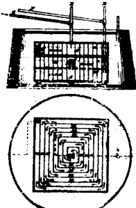
2341 Date's Carburetter.
