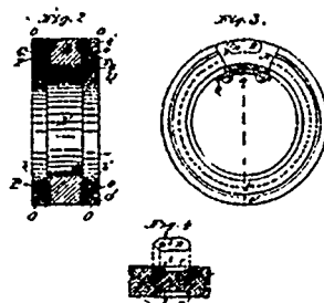
24294 St. John's Piston Packing.
