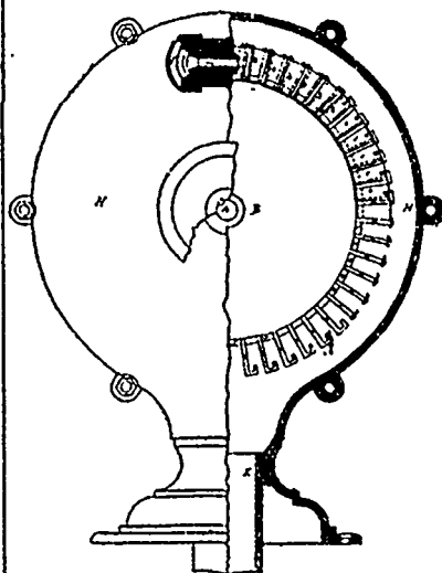
24291 Panet & Hallé's Water Motor.
