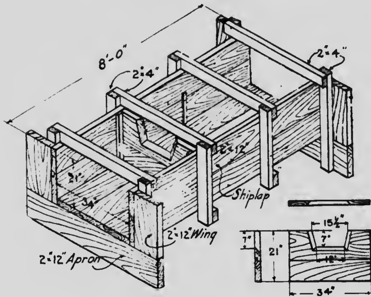
Fig. 3.—Trapezoidal weir-box.
