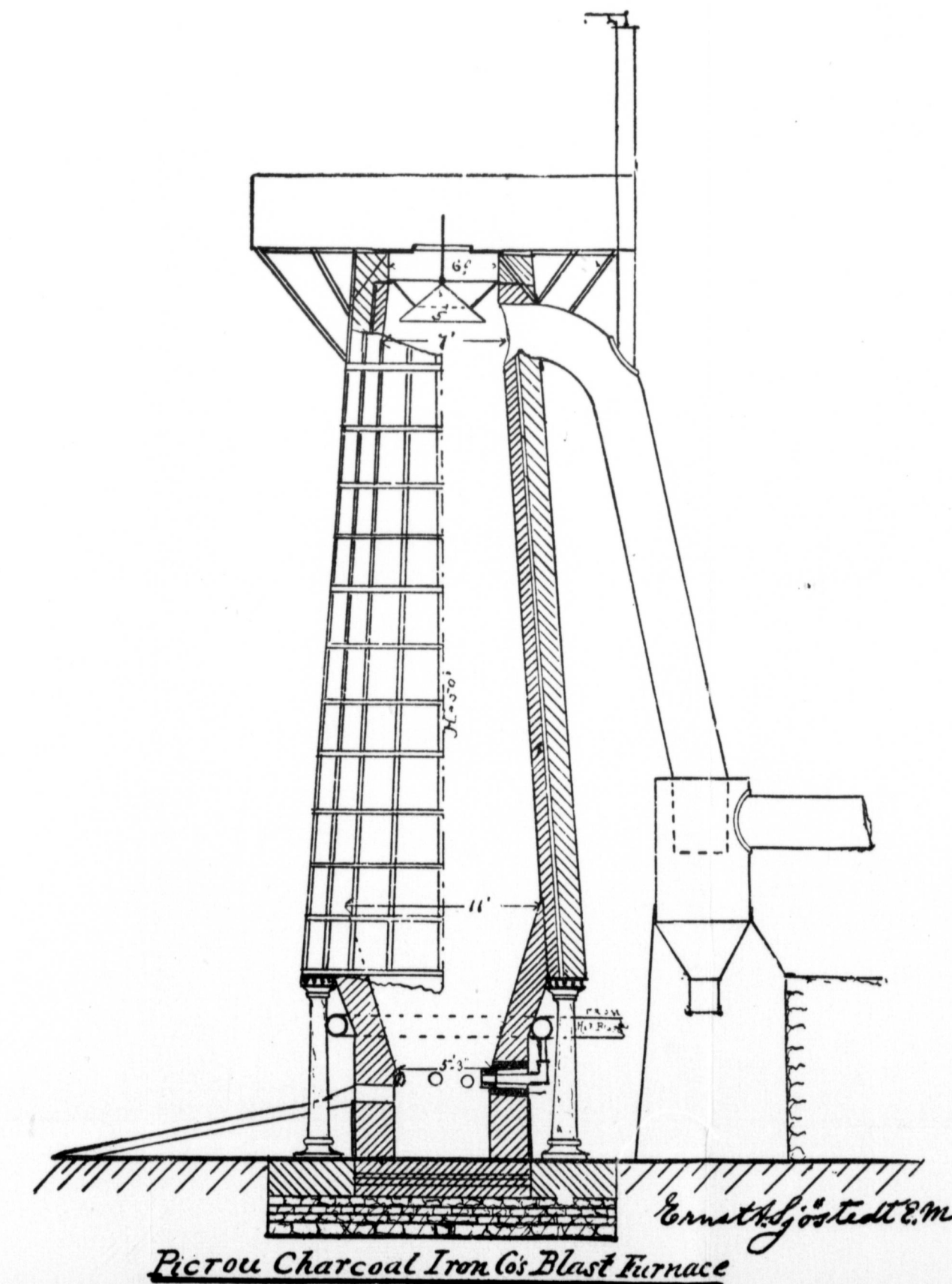
Plate IV.—Illustrating Mr. E. A. Sjostedt's Paper, "Notes on the Ores and Blast Furnace Plant of the Pictou Charcoal Iron Co. Ltd."
