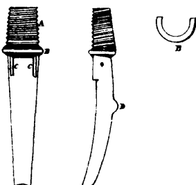
5743 Scott &amp; Delage's Improvements on Sap-Spouts.
