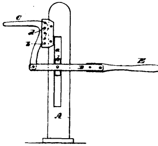
5732 Stanton's Waggon-jack.
