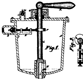
5738 Libbey's Liquid Meter.
