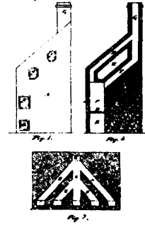
4411 Stephenson's Steel Tempering Oven.
