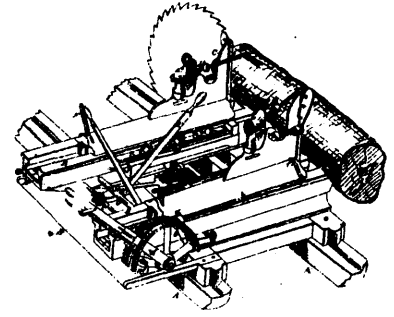
4418 Rodgers' Circular-saw Carriage.
