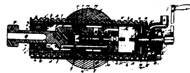
7481 Winchester &amp; Flagler's Improvements on Direct Acting Engines.
