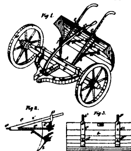
7478 Murphy's Improvements on Road Scrapers.
