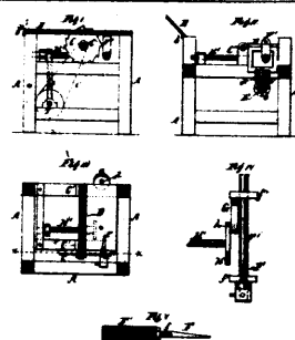
7475 Fisher's Sash Relishing Machine.
