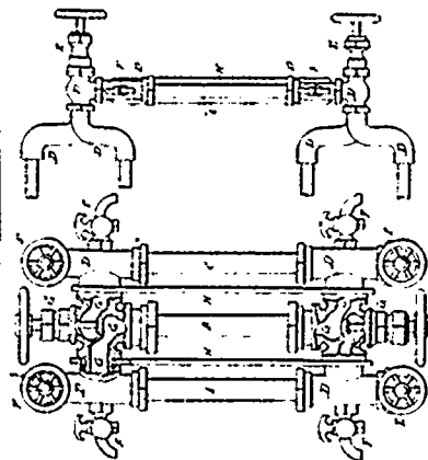
24814 Pyke's Water Gauge for Steam Boilers.
