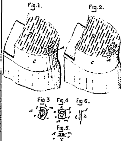
24820 Sanford's Heel Protector for Boots and Shoes.
