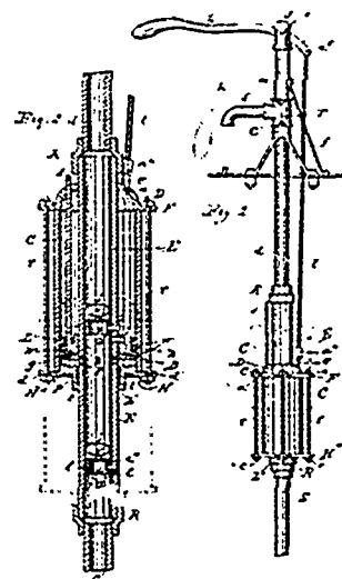
24817 Cloud's Force Pump.
