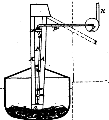
21795 Hayes' Grain Elevator.
