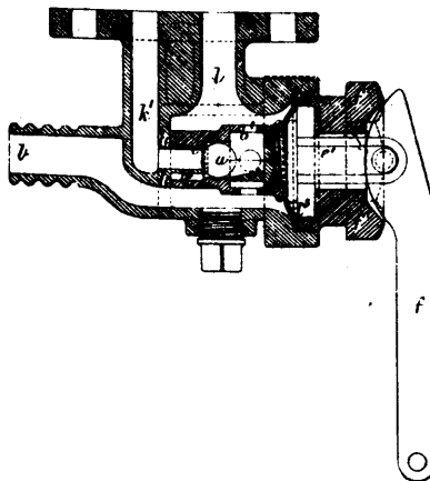
21791 Gresham's Automatic Vacuum Brake Apparatus.
