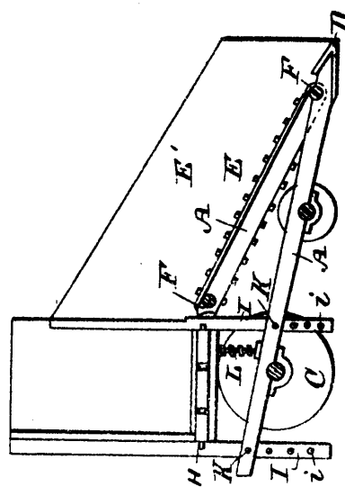
17375 Menze's Improvement in Snow Removers
