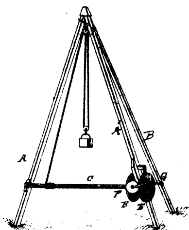
17373 Richardson's Improvement in Hoisting Gine
