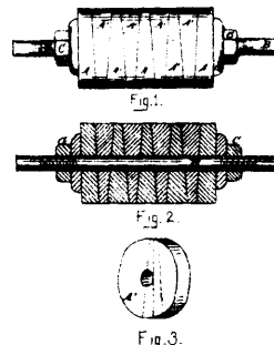
13485 Allen's Improvements in Wood Grinders for Making Paper Pulp.
