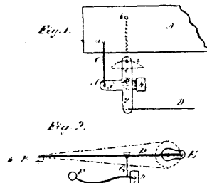
13492 McKenzie's Improvements on Fanning Mills.
