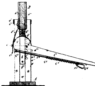
13487 Goodwin's Improvements on Lifting Jacks.
