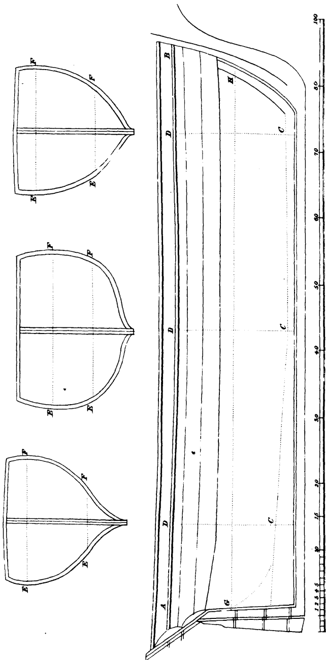
DIAGRAM ILLUSTRATIVE OF MEASURING VESSELS
