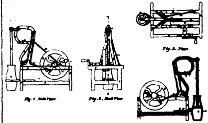
4619 Cole's Motive Power for Churns, &c.
