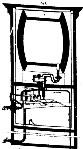
34966 Schoosing & Degremont's Coin Operated Liquid Vending Apparatus.
