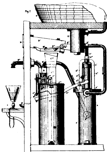
34967 Schoosing & Degremont's Coin Operated Liquid Vending Apparatus.
