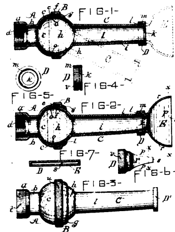
34968 Pearsall's Hose Nozzle.
