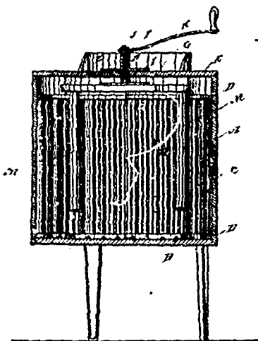
25355 Greuter's Washing Machine.
