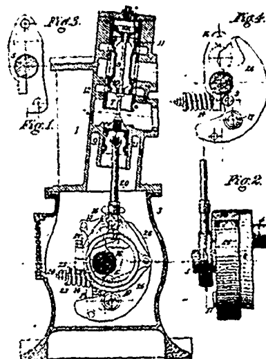
25356 Rito's Steam Engine Governor.
