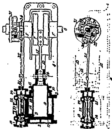
25364 Westinghouse's Steam Engine.
