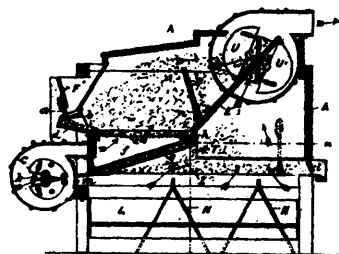
7581 Palmer's Improvements on Middlings Separators.
