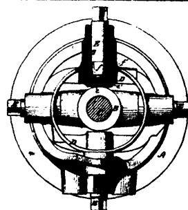
7588 Otis' Oscillating Joint for Machinery.
