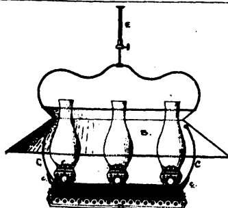
7590 May's Improvements in Coal Oil Lamps.
