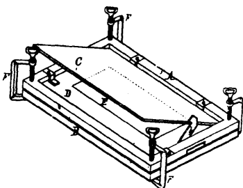
7580 Long's Process of Enamelling Photographs.
