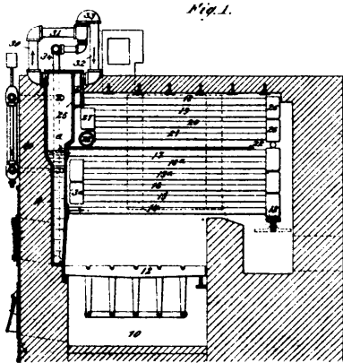
33813 Dietrich's Steam Boiler.
